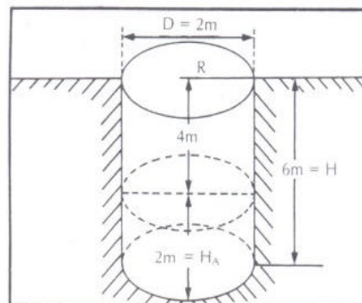
Figura 1 Cisterna circular
